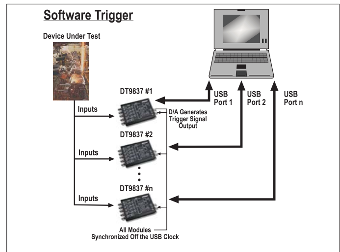
Figure 8. Using a software call to generate a trigger signal on one D/A output tied to all external trigger lines synchronizes the start of conversion for all modules.
