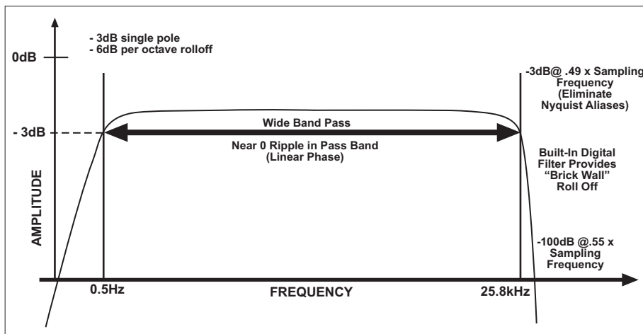
Figure 6. The DT9837 provides software selectable AC and DC coupling. When AC coupling is selected, the modules provide zero ripple in the wide pass band and excellent "brick wall" anti-alias filters eliminating unwanted high frequency interference.
