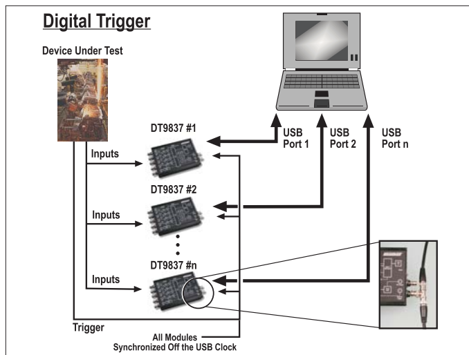
Figure 7. Multiple DT9837 modules can be triggered simultaneously by connecting all modules to a shared external trigger input.
