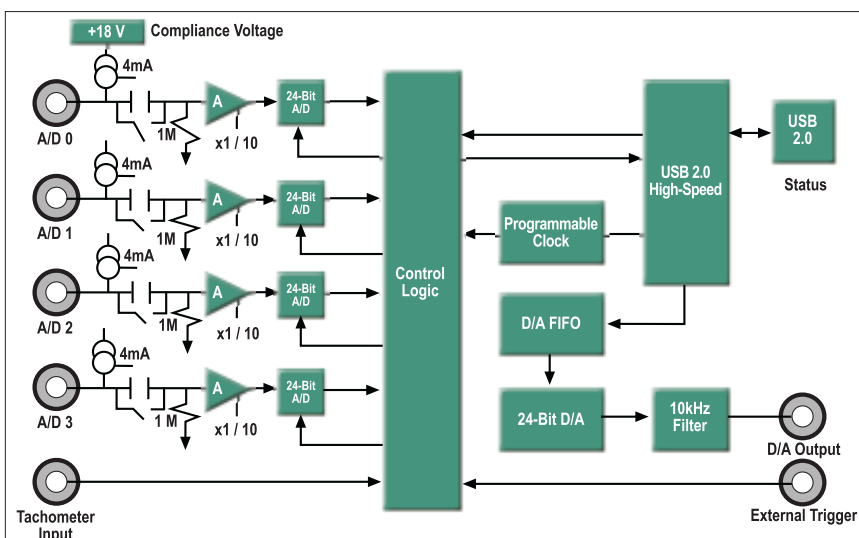
Figure 2. The DT9837 is a high performance, multifunction data acquisition module for USB that provides A/Ds with IEPE capability, one waveform D/A, a tachometer input, and simultaneous operation of all subsystems.
