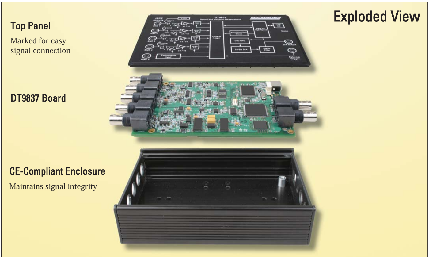
Figure 4. The DT9837 board is encased in a rugged, metal enclosure to ensure CE-compliance and maintain signal integrity.
