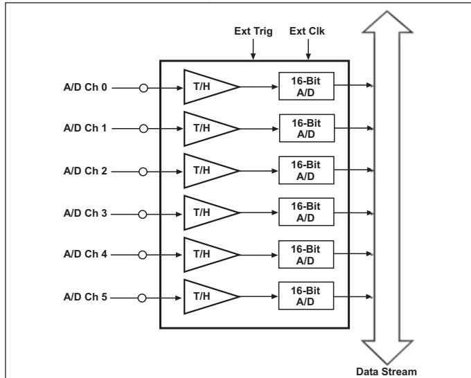
Figure 10. The DT9816 modules feature six, independent, successive-approximation A/D converters with track-and-hold circuitry. Each converter uses a common clock and trigger for simultaneous sampling of all six analog input signals. The throughput rate varies depending on the model you choose.
