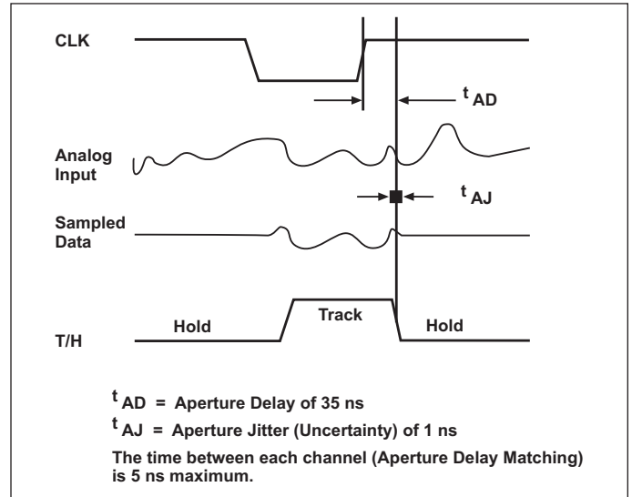
Figure 11. The A/D design of the DT9816 modules feature built-in accuracy. A maximum aperture delay of 35 ns (the time that it takes the A/D to switch from track to hold mode) is well matched at 5 ns across all six track-and-hold circuits, virtually eliminating the channel-to-channel skew that is associated with multiplexed inputs. A maximum aperture uncertainty of 1 ns (the jitter or variance in aperture delay), virtually eliminates phase noise in your data.
