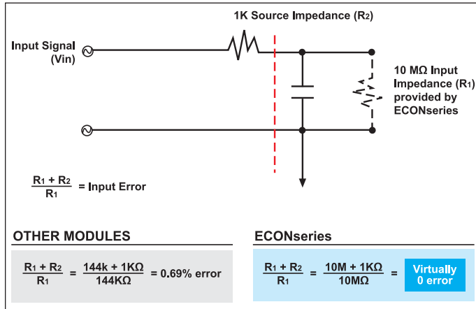
Figure 5. The ECONseries provides 10 MOhms of input impedance for virtually error-free analog input measurements.
