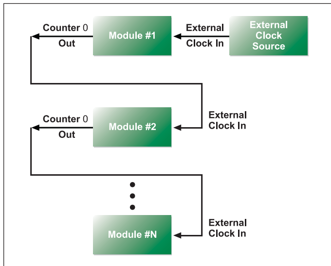
Figure 13. You can synchronize the analog I/O operations of multiple modules by connecting them together.
