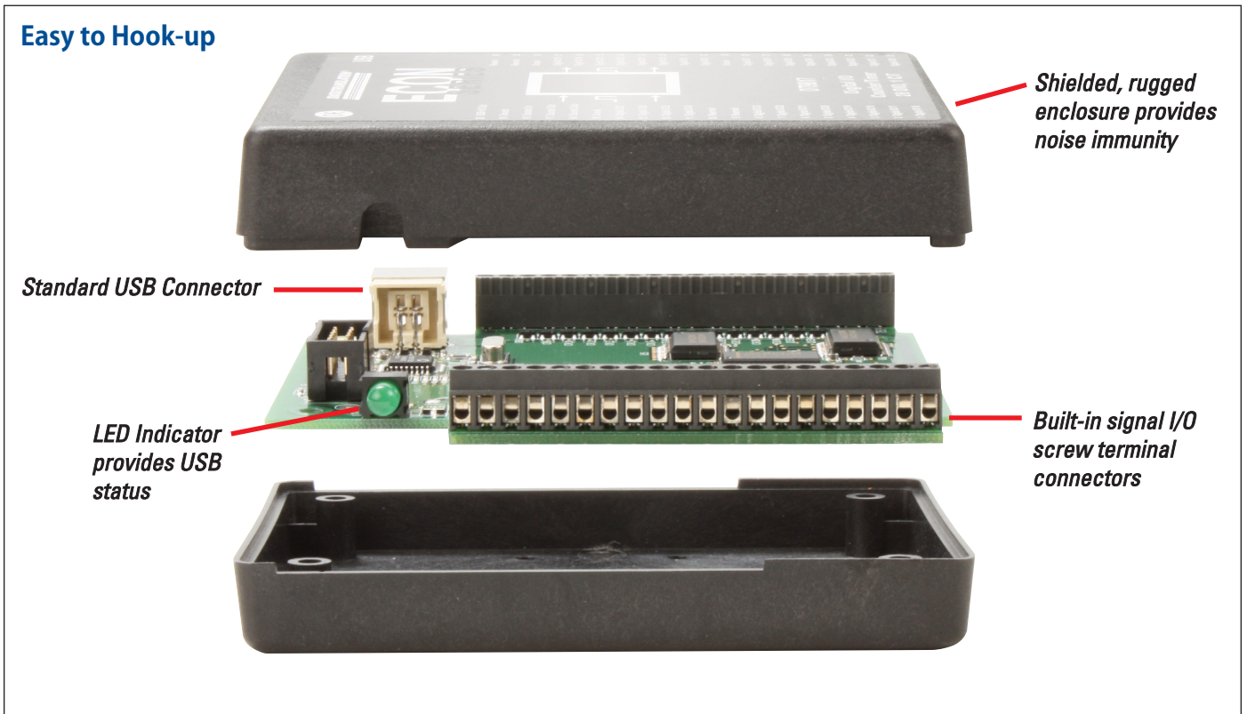
Figure 4. ECONseries modules provide easy signal and USB connections in a shielded, rugged enclosure.
