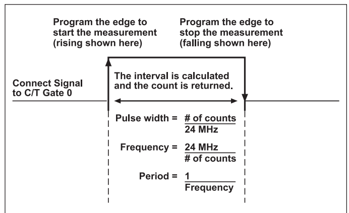
Figure 9. Programmable edges allow you to use the counter/timer of an ECONseries module to measure the pulse width, frequency, and period of a signal.
