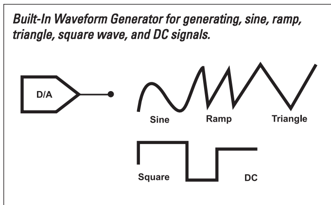
Figure 8. The DT9812-2.5 V, DT9812-10V, DT9813-10V, and the DT9814-10V modules provide 2 waveform DACs for generating sine, ramp, triangle, square wave, and DC signals.
