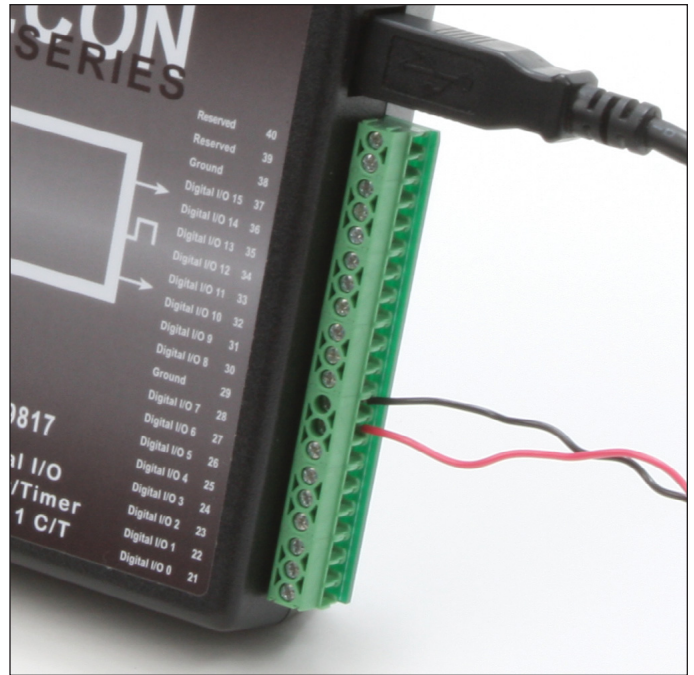
Figure 3. Connect sensors directly to the screw terminal of the module. Screw terminals can accept AWG 26 to AWG 16 size wire.
