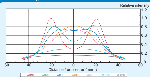
UDR-30R60 Light distribution at various WD
