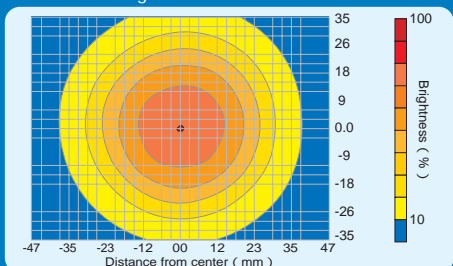
UDR-30R60 Light distribution at WD 40mm
